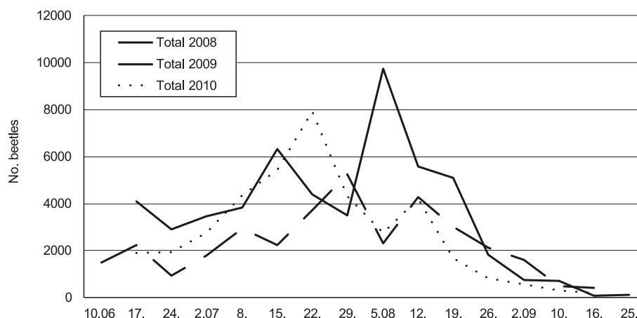
Fig. 2. Total seasonal activity of ground beetles in (a) Budziszów and (b) Głuchów in the 2008–2010
