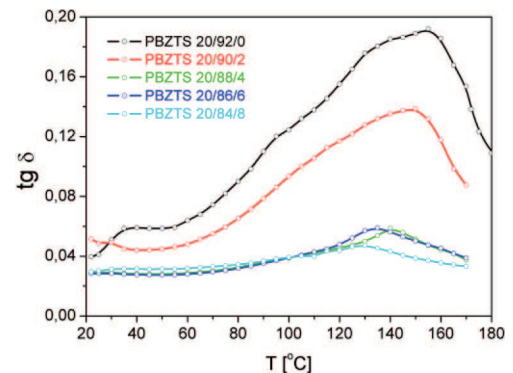
Fig. 5. Dependency \text{tg}\delta(T) for investigated ceramic samples
