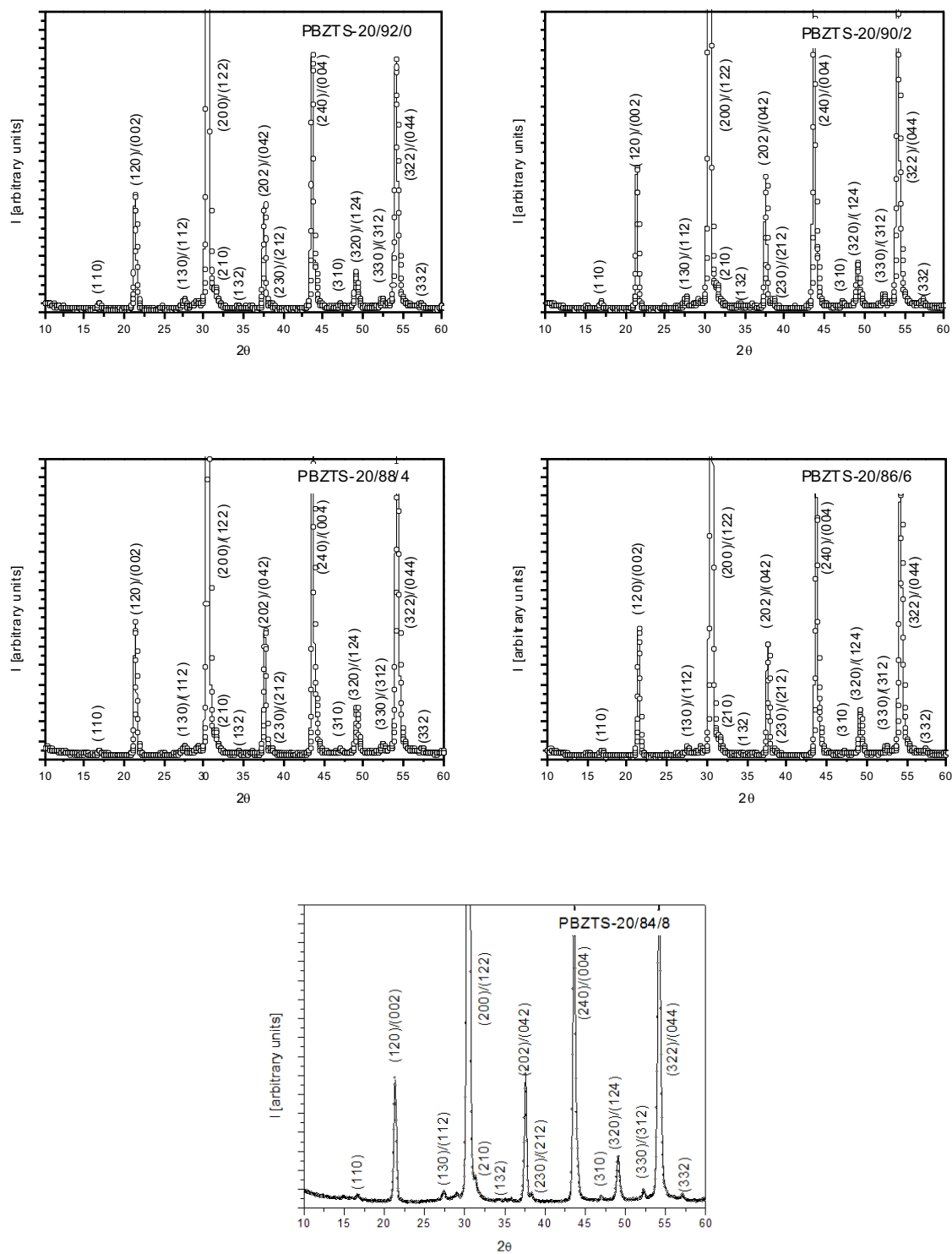
Fig. 3. XRD diffraction patterns of PBZTS ceramics powders at room temperature
