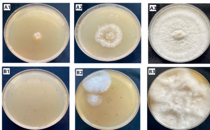
Fig. 1. Antifungal activity of Bacillus velezensis NC318 crude extracts on Sclerotium rolfsii mycelial growth (A1 – 50 µl crude extracts, A2 – 10 µl crude extracts and A3 – 50 µl methanol – control) after 5 days of incubation at 30°C and sclerotia germination (B1 – 50 µl crude extracts, B2 – 10 µl crude extracts and B3 – 50 µl methanol – control) after 10 days of incubation at 30°C
