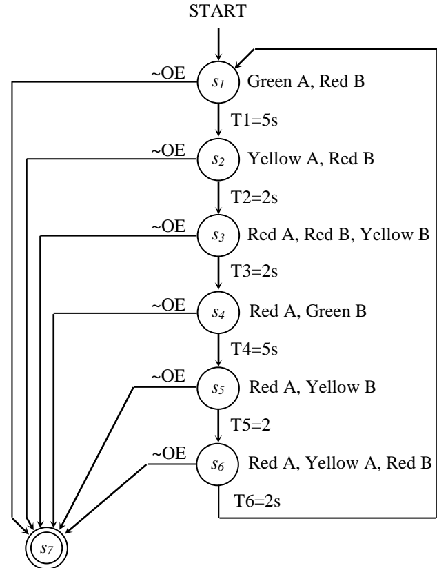
Fig. 3. FSM graph of streetlights control.
