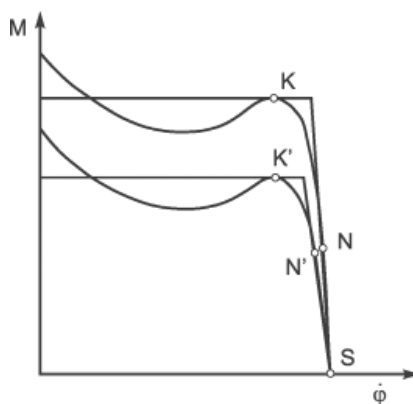
Fig. 2. Actual and approximated mechanical characteristic of asynchronous motor for supply with electricity directly from power mains
