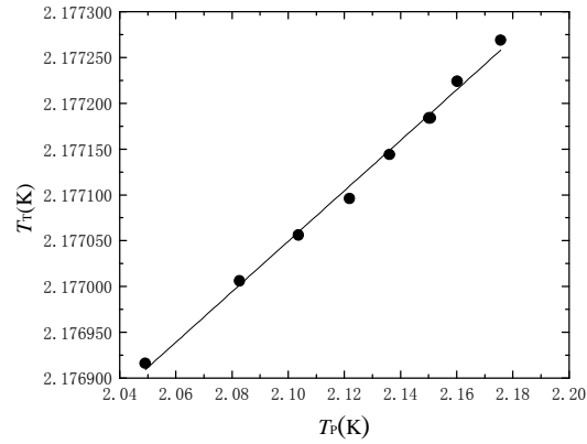
Fig. 6. A typical plot of T_T versus T_p for the sealed-cell L2.
