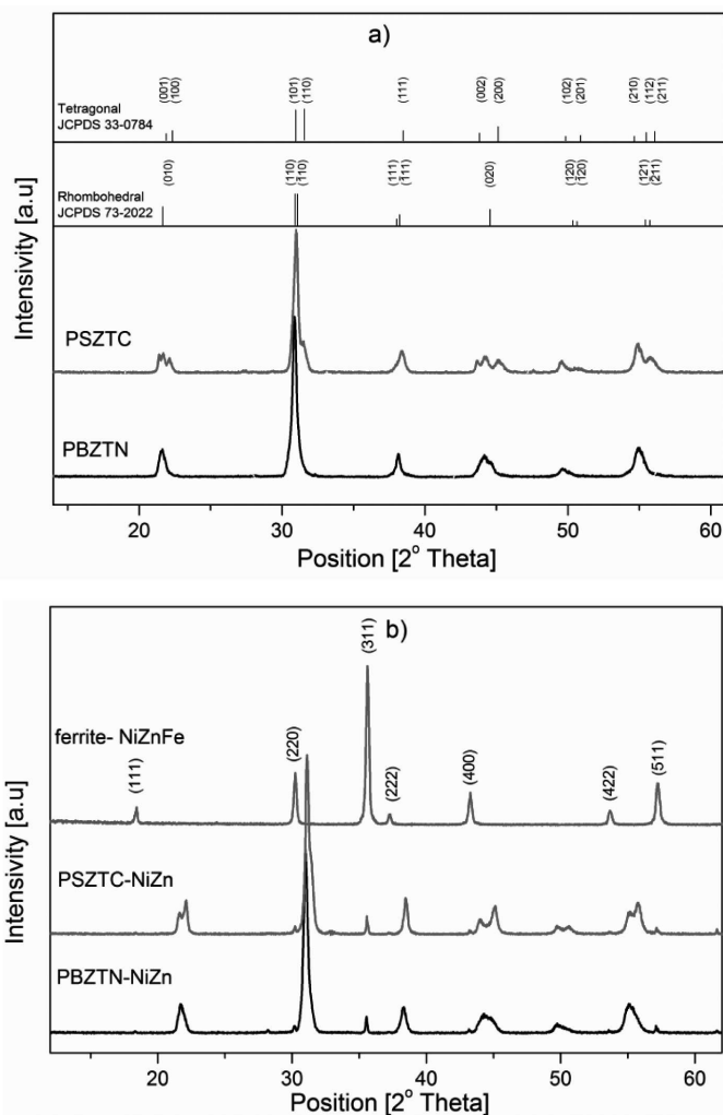
Fig. 1. 1 X-ray spectra of the PZT type powders (a) and PZT-NiZn composites (b)
