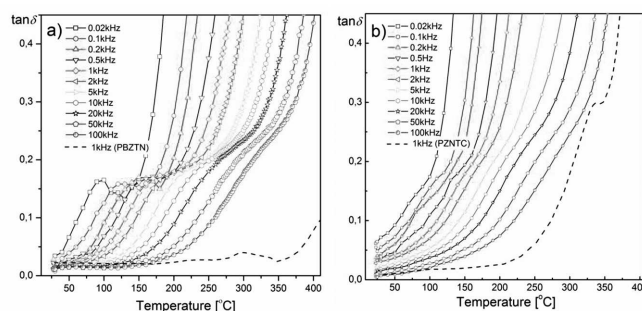
Fig. 5. Temperature relations of the \tan \delta for composite: a) PBZTN-NiZn, b) PSZTC-NiZn (heating)
