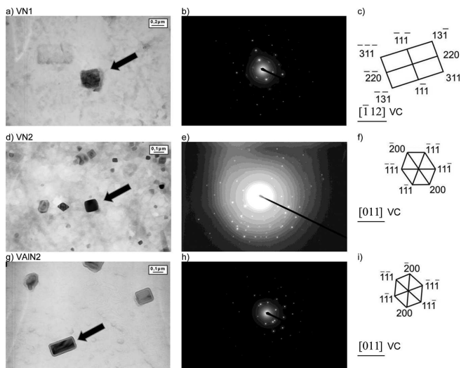
Fig. 6. Precipitate images (a, d, g), diffraction patterns (b, e, h) and solutions of diffraction patterns (c, f, i) of steels VN1 (a, b,c), VN2 (d, e, f) and VAIN2 (g, h, i)
