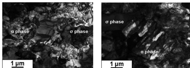
Fig. 4. The microstructure and point diffraction from the surface layer of deformed samples at 725 (a) and 850°C (b), TEM. The grains of \sigma phase are dark and without dislocations. The grains of \alpha phase are white and reveal a high density of dislocations
