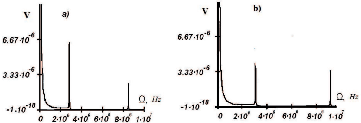
Fig. 6. Dependences of the photoacoustic signal amplitude on the modulation frequency \Omega at different geometric parameters of the sample–piezoelectric transducer system: a) \ell = 5,5 \cdot 10^{-3} m , for \ell = const b) \ell_1 = 5,5 \cdot 10^{-4} m , for \ell = const
