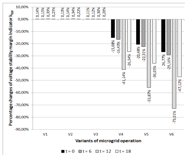
Fig. 10. Percentage changes in the indicator k_{QU} value of node N20 depending on the chosen microgrid operation variant in relation to V0 variant
