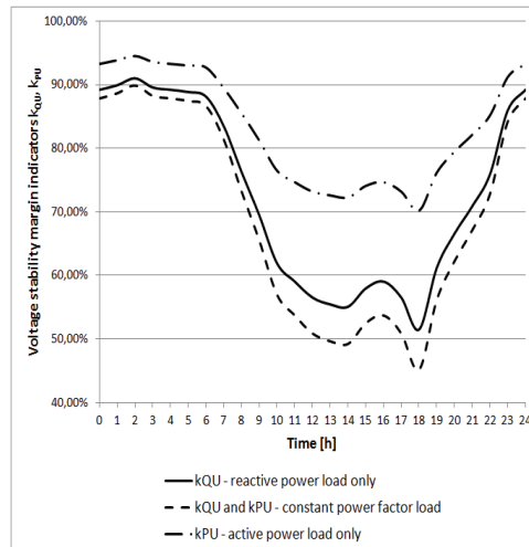
Fig. 9. Daily changes k_{QU} and k_{PU} indicators in node N35 – variant V6
