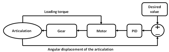
Fig. 5. Block diagram of the control loop for the drive unit of the articulation of the device
