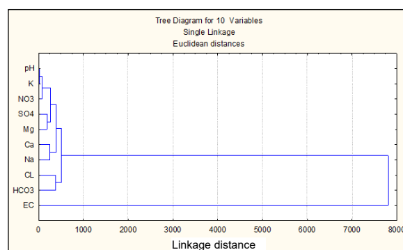
Fig. 4. Cluster dendrogram for variables; source: own study
