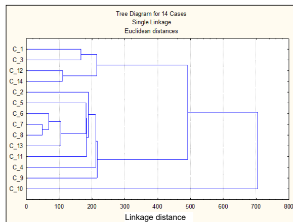
Fig. 5. Cluster dendrogram for water samples; source: own study
