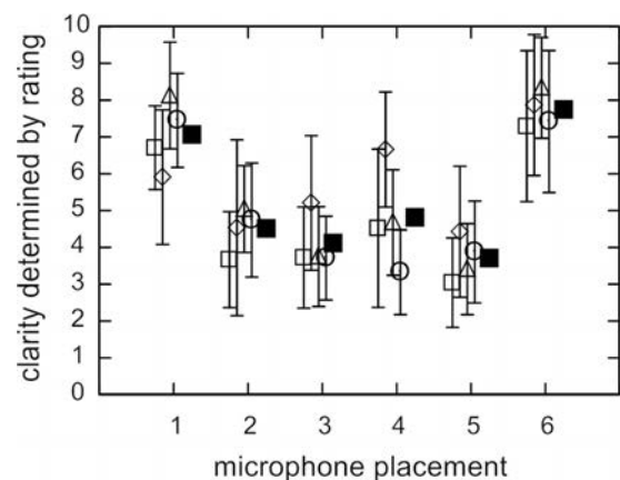
Fig. 2. Results of rating of sound clarity on a scale from 0 to 10. Open symbols show arithmetic means of 12 judgments obtained for individual musical excerpts: Waltz (piano) – squares, Fantasie-Improptu (piano) – diamonds, Obertas (violin) – triangles, Romanian Dance (violin and piano) – circles. Error bars represent the standard deviation of the mean. Filled squares show arithmetic means calculated across musical excerpts.
